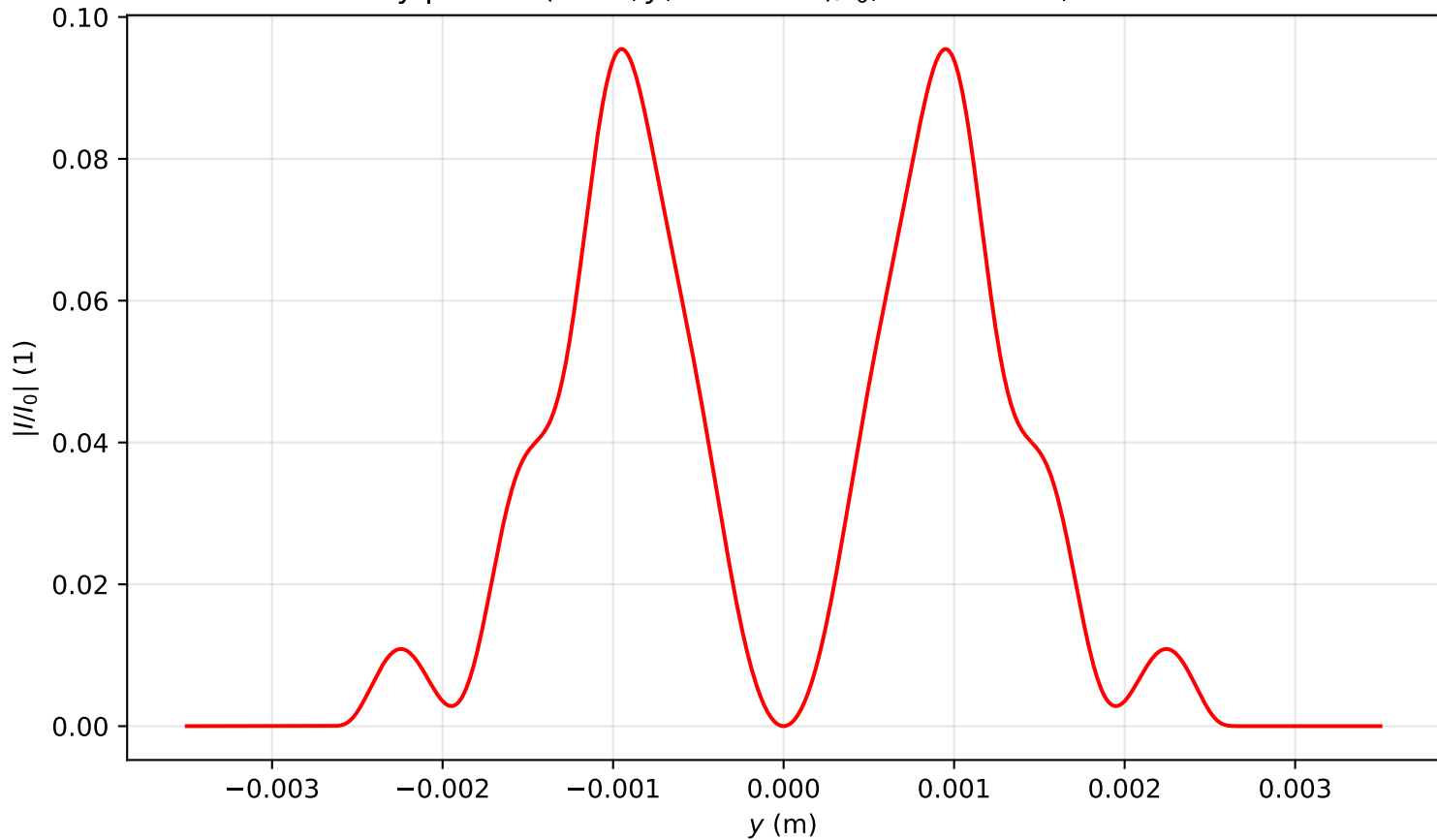
Intensity profile I(x=0, y, z=3.901)/I_0 , P_{in}=4.0P_{cr} , artificial time
